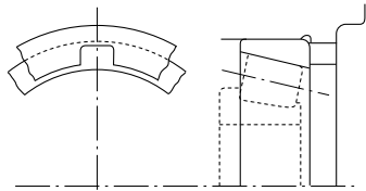
Fig. 14.11 Removal Notches
